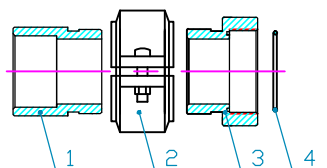
GROOVED CONNECTORS WITH COUPLING
